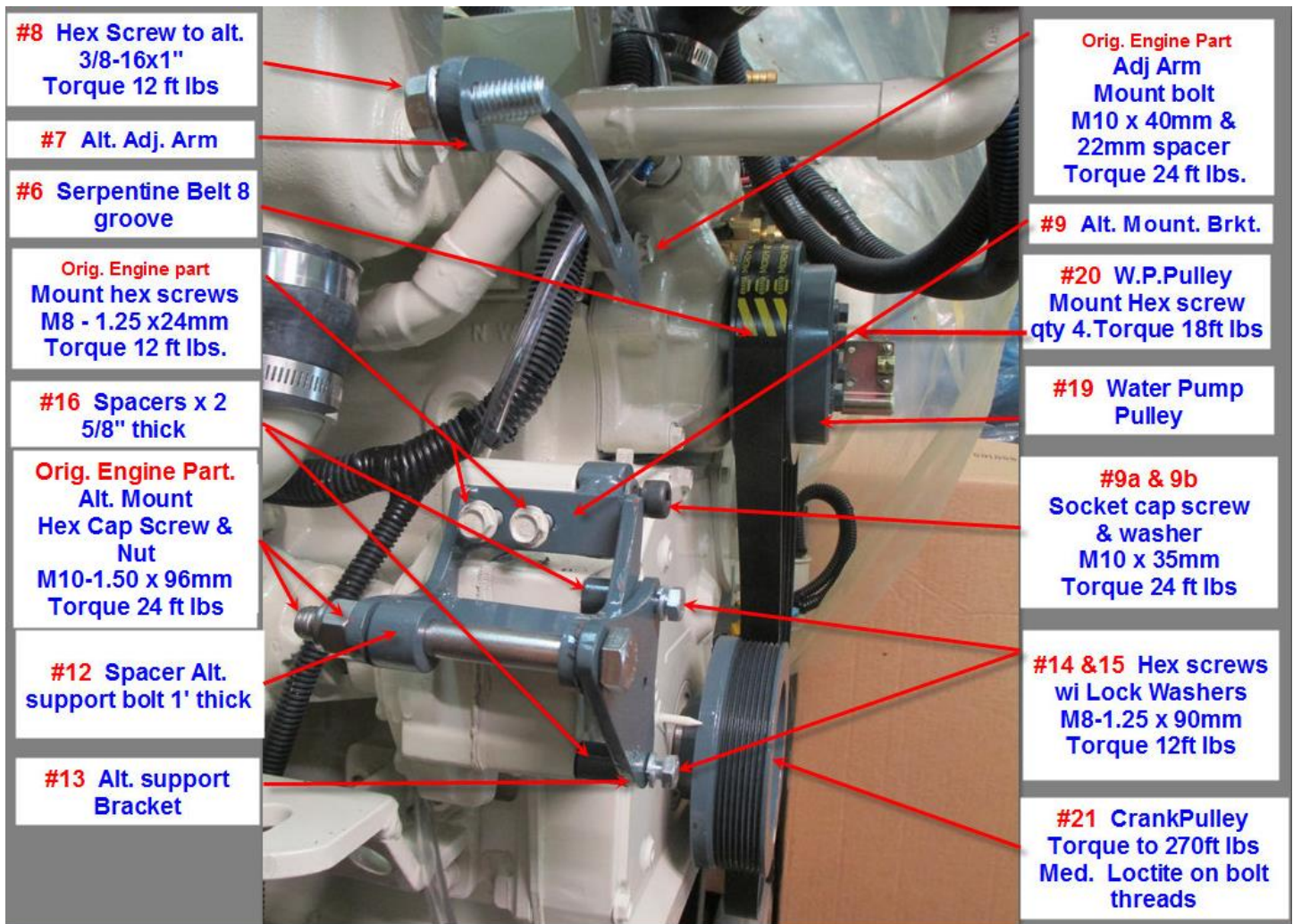
REFERENCE NUMBERS, FASTENER SIZES, AND TORQUE SETTINGS
