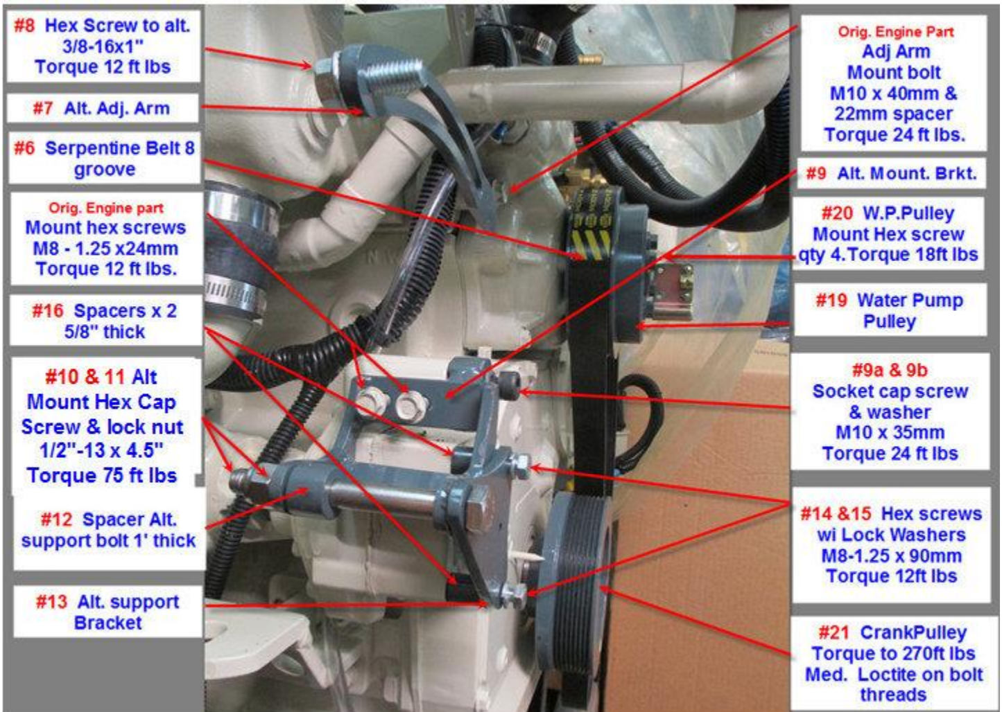
REFERENCE NUMBERS, FASTENER SIZES, AND TORQUE SETTINGS
