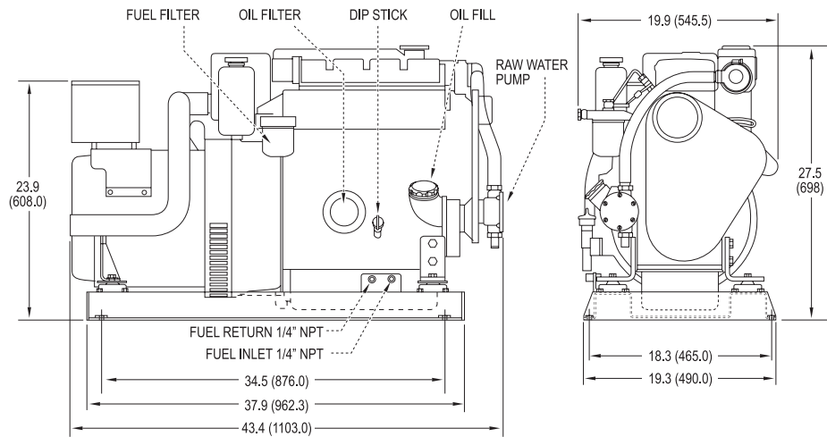
M844LW3 Overall Dimensions L x W x H: 43.4 x 19.9 x 27.5 inch (1103 x 545.5 x 698 mm) Dimensions given in inches (mm). Dimensions subject to change without notice. Contact dealer or visit www.northern-lights.com for most current installation drawings.
