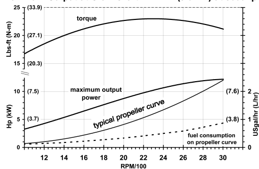
Maximum Output at Crankshaft = 12 HP (9.0 kW) at 3000 rpm
